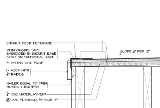
5 BALCONY DETAIL AT EDGE 3/4" = 1'-0"
