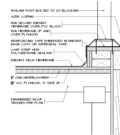
3 ROOF EDGE DETAIL 3/4" = 1'-0"
