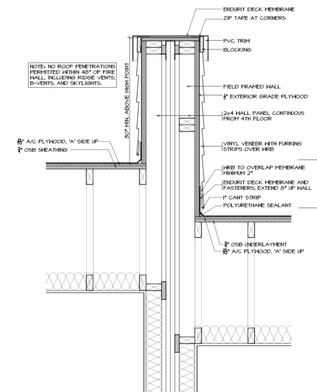
11 ROOF PARAPET WALL BETWEEN UNITS 1/2" = 1'-0"
