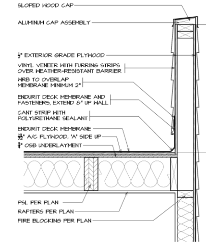
4 PARAPET DETAIL AT FRONT 1/2" = 1'-0"
