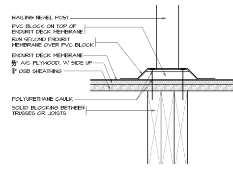
6 RAILING ATTACHMENT DETAIL 3/4" = 1'-0"
