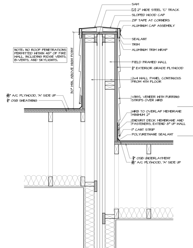
10 ROOF PARAPET WALL BETWEEN UNITS 1/2" = 1'-0"
