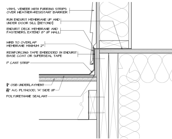
2 BALCONY DETAIL AT WALL 3/4" = 1'-0"
