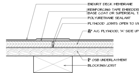
7 PLYWOOD JOINT 3/4" = 1'-0"
