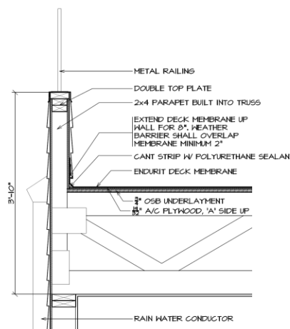
8 PARAPET DETAIL AT REAR 1" = 1'-0"
