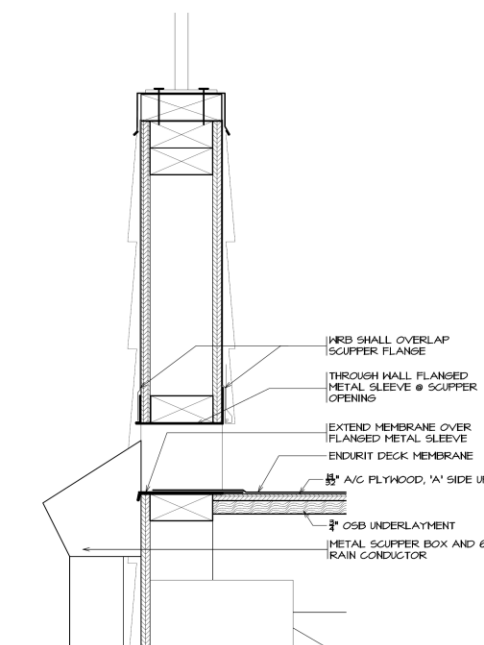
9 DETAIL AT SCUPPER 3/4" = 1'-0"
