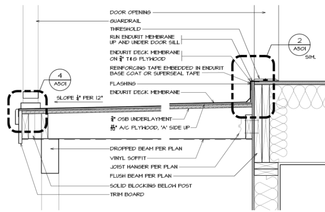
1 BALCONY DETAIL AT UNIT 1/2" = 1'-0"
