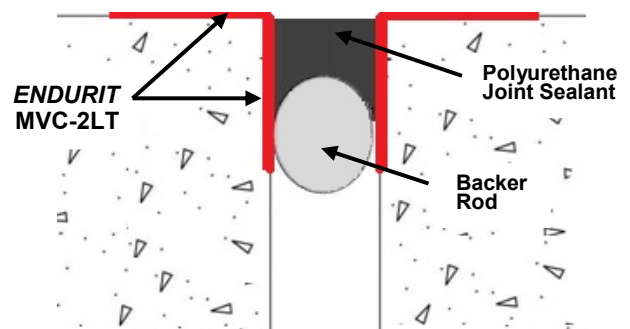
Expansion Joint Detail with ENDURIT MVC-2LT
