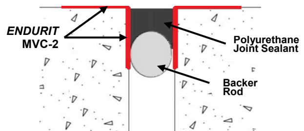
Expansion Joint Detail with ENDURIT MVC-2
